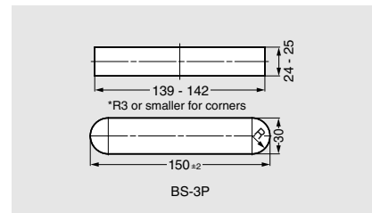
Cut Out Dimensions
