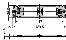
Cut Out Dimensions
