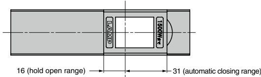
When fully open (DMC-1-MC)
