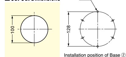
Installation position of Base ②
