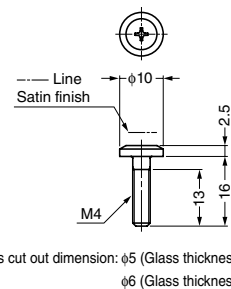
⑤ Truss head screw M4×16
