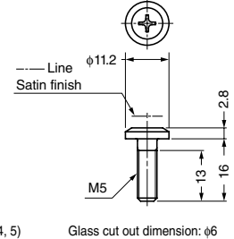
⑥ Truss head screw M5×16
