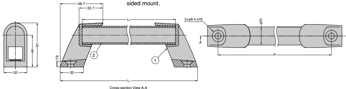
Cross-section View A-A
