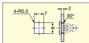
Cut Out Dimensions (Strike for Snap-in)
