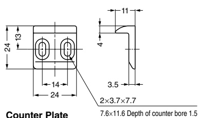
Counter Plate
