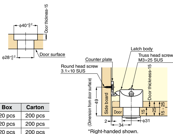
Latch Body and Counter Plate
