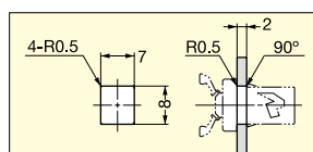
Cut Out Dimensions for body
